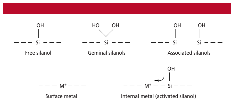
Figure 3: The silica surface. (Reprinted from reference 1 with permission.)
